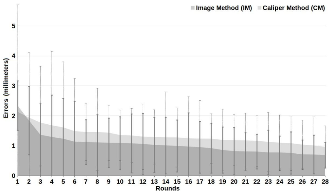
Figure 5. Mean error and its standard deviation for each of the 28 measurement rounds for the 30 plants, for both methods, sorted from highest to lowest mean error.
